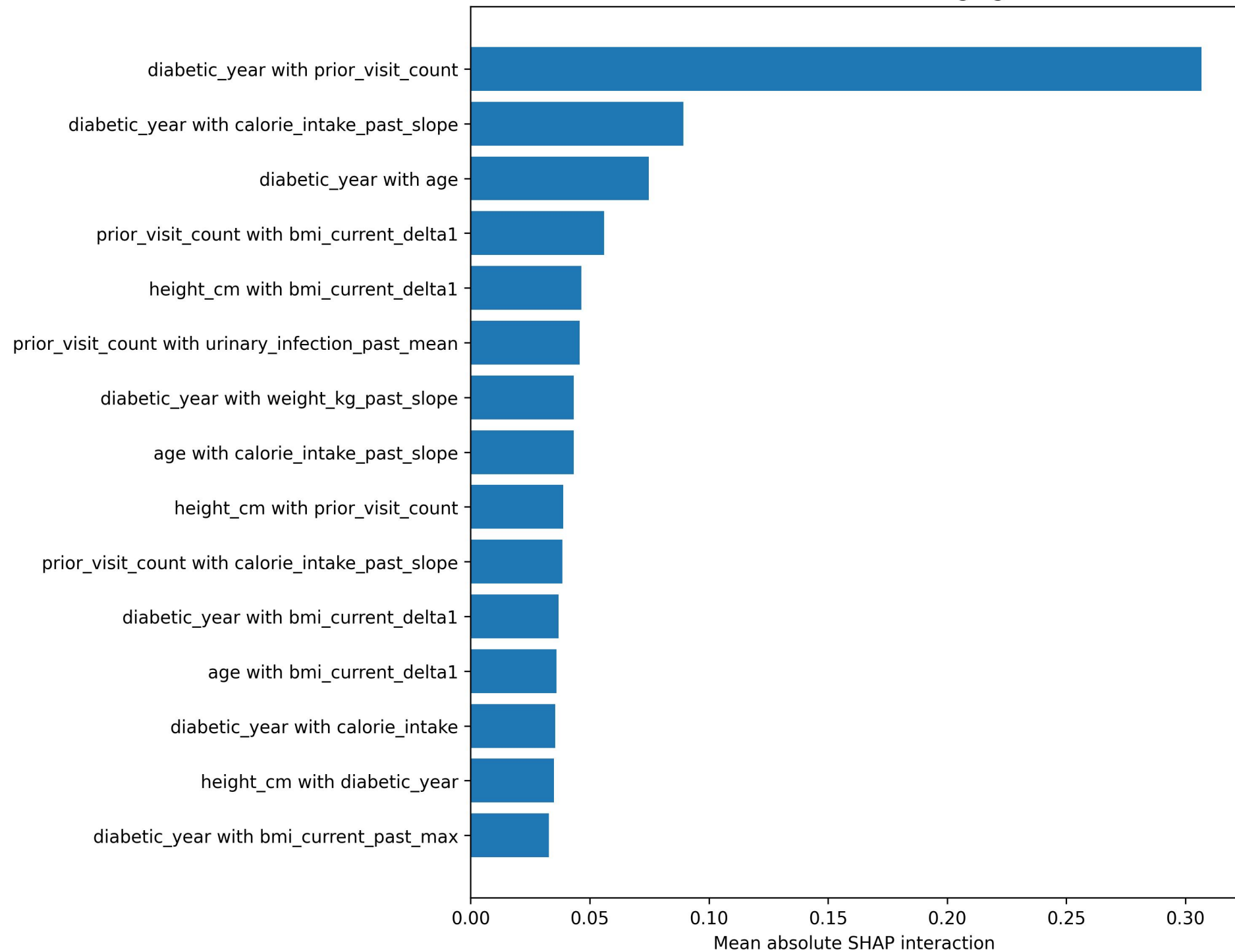
Stable SHAP interactions: lightgbm
